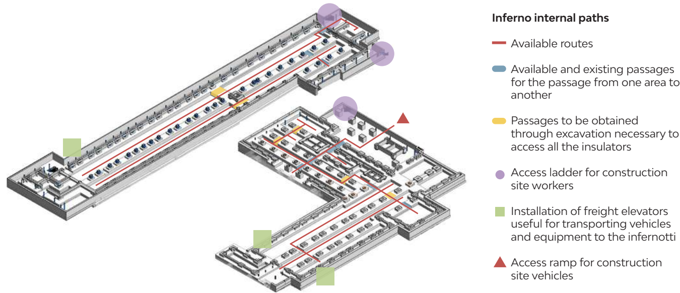
Access methods and sequence of laying of insulators
